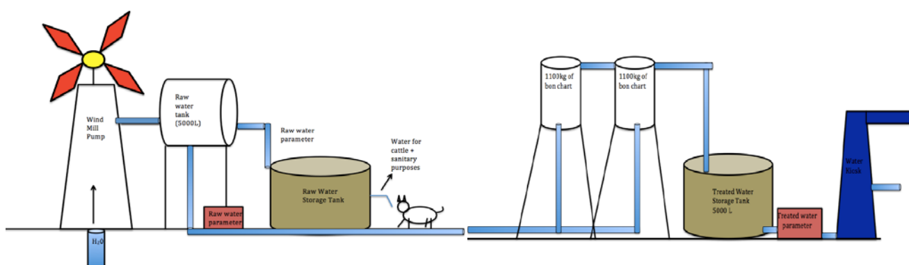
Figure 5 Community bone char defluoridation scheme
