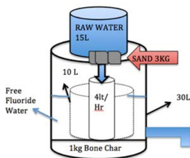
Figure 4 Household bone char
